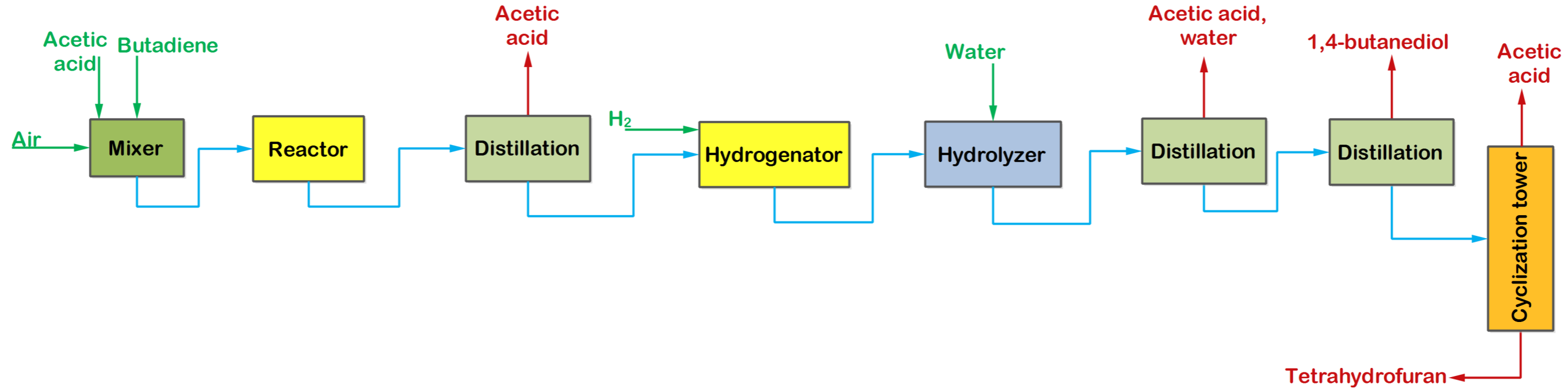
Figure: Manufacture of tetrahydrofuran from butadiene acetoxylation
